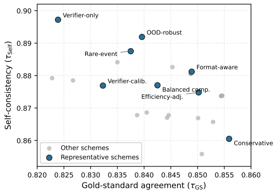
Figure 4: Gold-standard agreement vs. self-consistency for 25 categorical schemes at N=1 on the Combined benchmark. Blue markers indicate the 8 representative schemes; gray markers show the remaining 17. Schemes in the upper-left are self-consistent but deviate from \text{Bayes}_{\mathcal{U}}@80 ; those in the lower-right closely track the gold standard but are less stable across single-trial draws.
