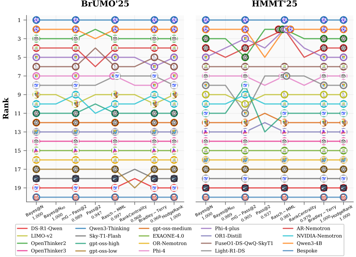
Figure 1: Agreement between each method’s full-trial ranking and the gold standard. Kendall’s \tau_b is computed between each method’s ranking (at N = 80 trials) and \text{Bayes}_{\mathcal{U}}@80 on an easier benchmark (BrUMO’25, left) and the hardest benchmark (HMMT’25, right). On BrUMO’25, multiple methods achieve near-perfect or perfect agreement: \text{Bayes}_{\mathbf{R}_0}@N and HodgeRank reach \tau_b = 1.0 , while Rasch MML achieves 0.997. On HMMT’25, Bradley–Terry and HodgeRank maintain perfect agreement ( \tau_b = 1.0 ), but \text{Bayes}_{\mathbf{R}_0}@N drops to 0.989 and Pass@2 falls to 0.937. This divergence is consistent with the lower greedy–sampling alignment observed on harder benchmarks (Section 3.4).
